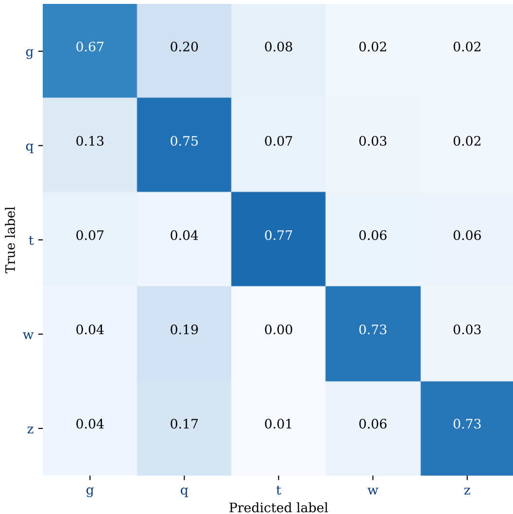
Confusion Matrix of Jet-tagger: QKeras
